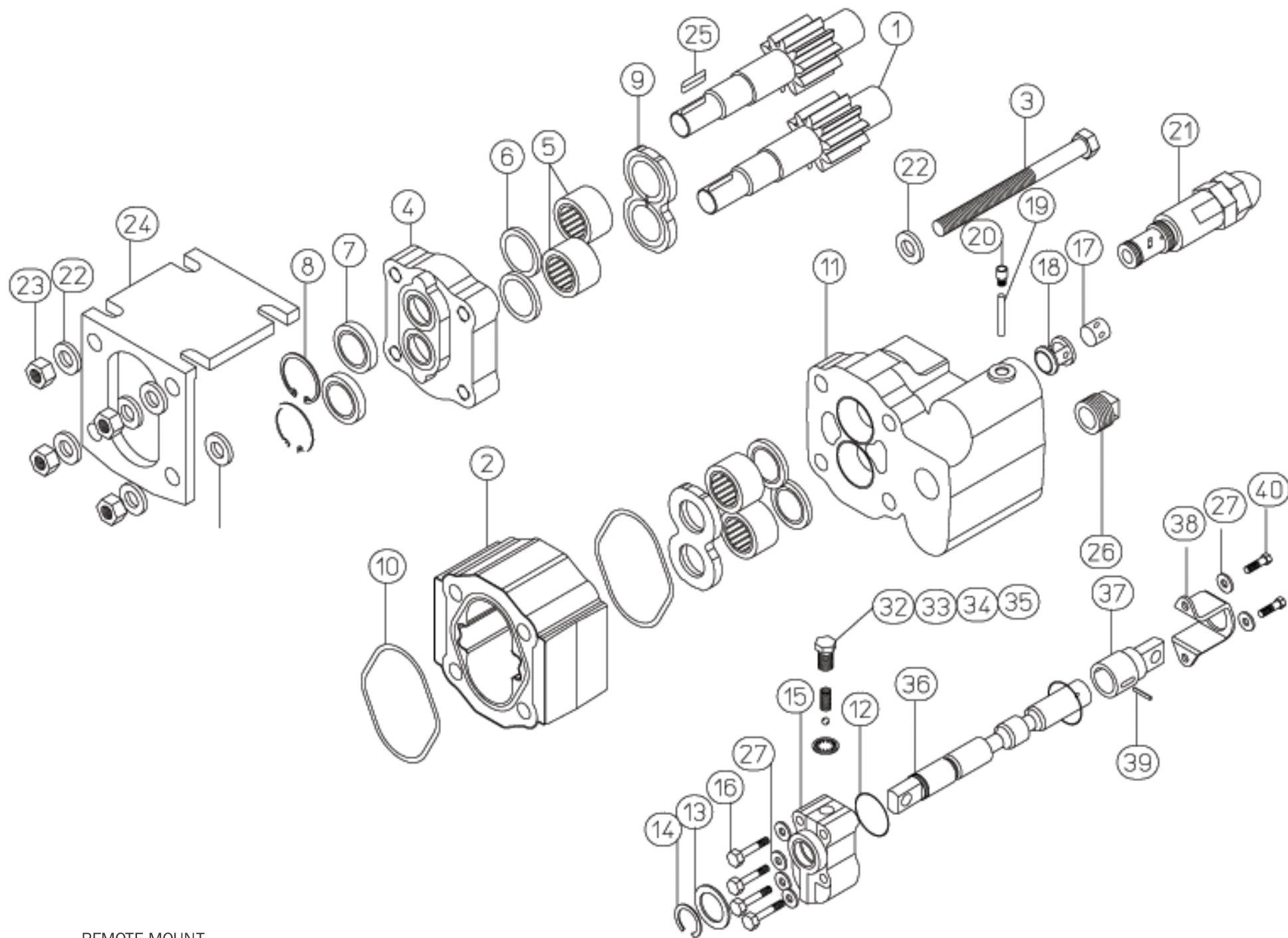
REMOTE MOUNT
