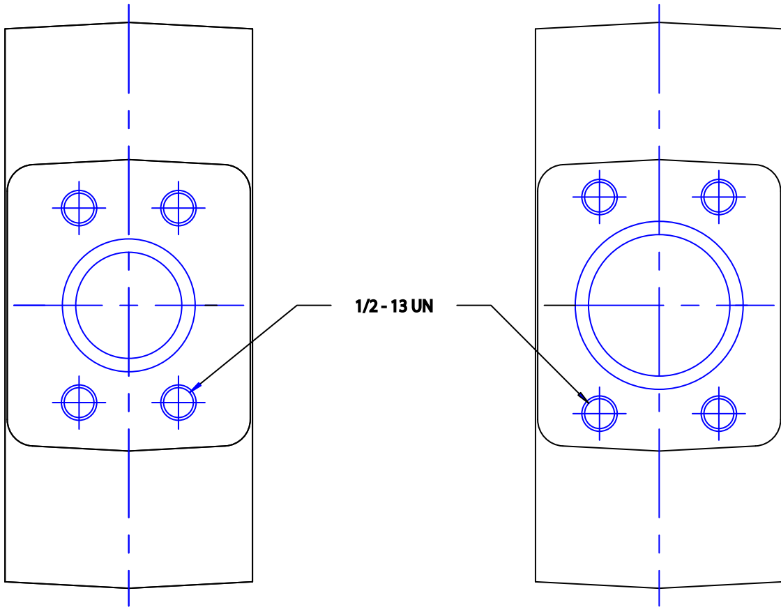
1-1/2 INCH
